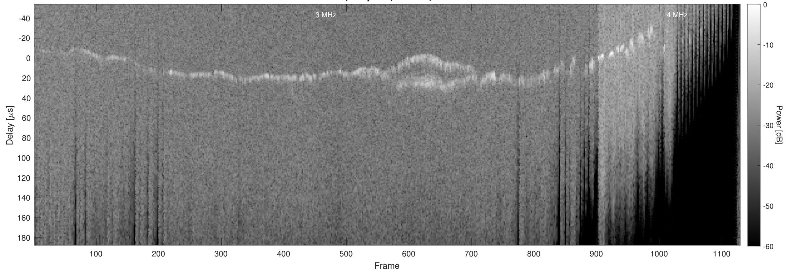
Orbit 14005, Chapman, Window, Channel 2
