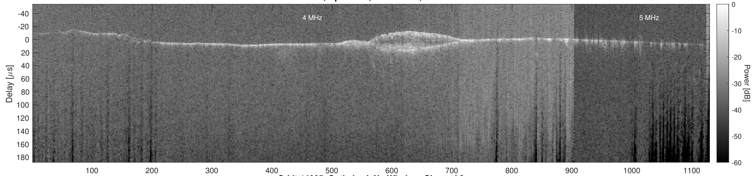
Orbit 14005, Optimized, No Window, Channel 2
