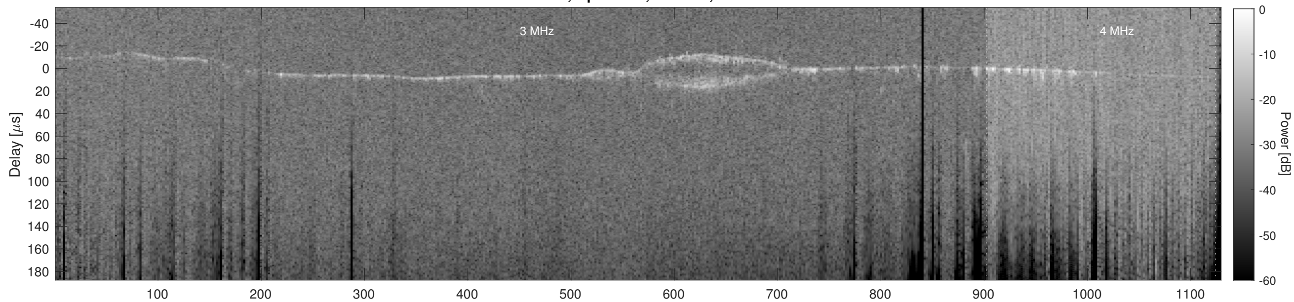
Orbit 14005, Cluttergram
