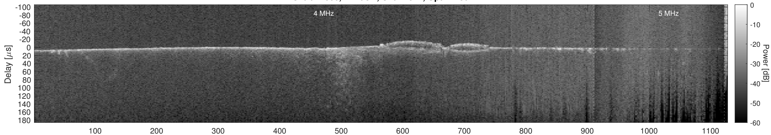
Orbit 14006, Cluttergram
