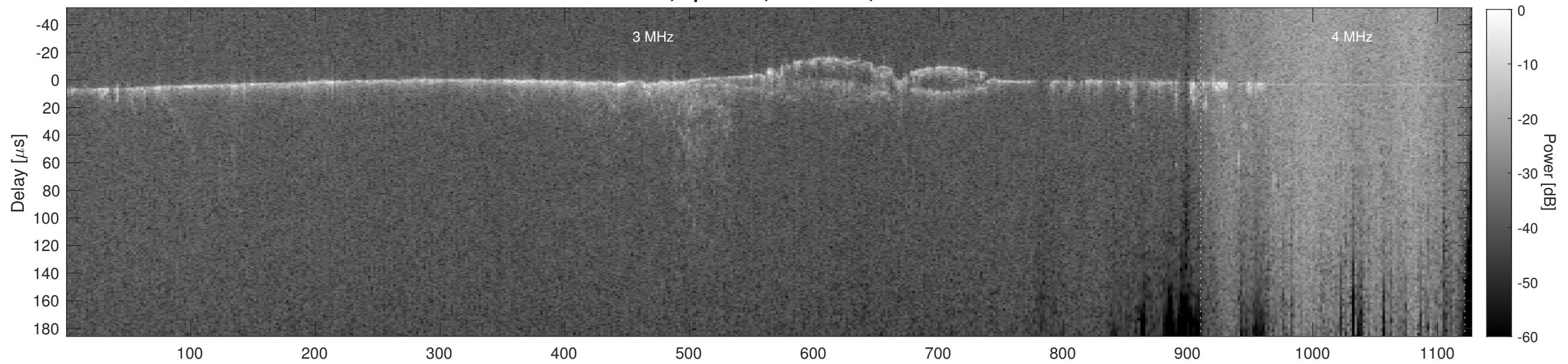
Orbit 14006, Cluttergram
