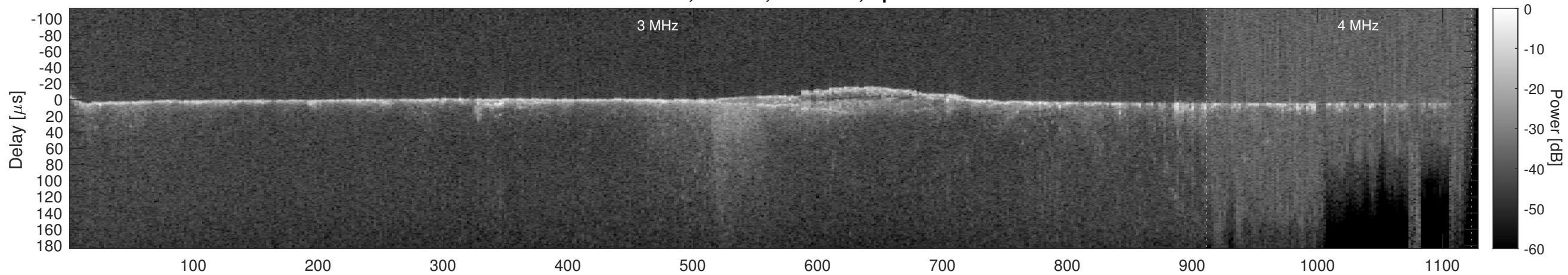
Orbit 14010, Cluttergram
