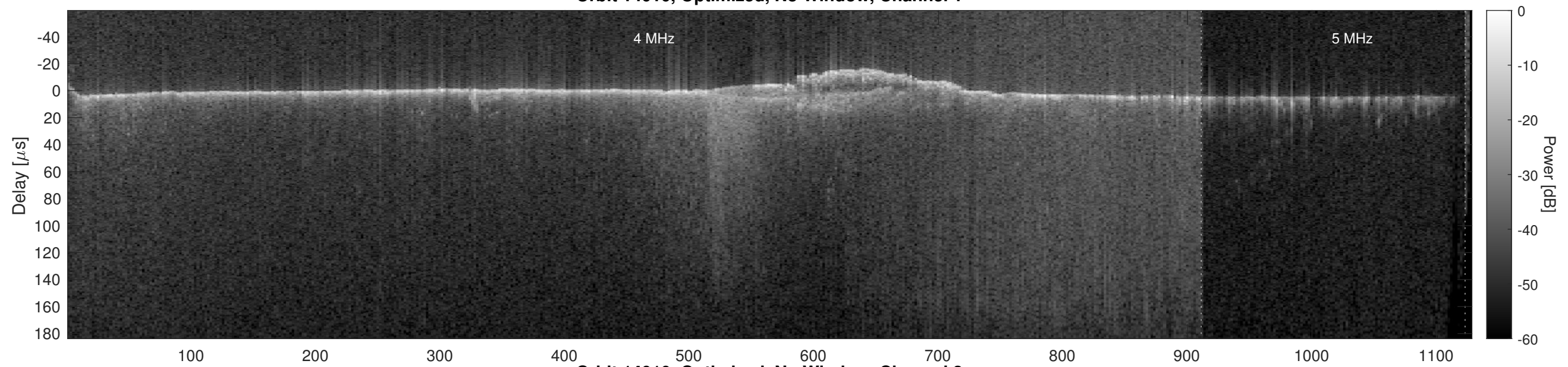
Orbit 14010, Optimized, No Window, Channel 2
