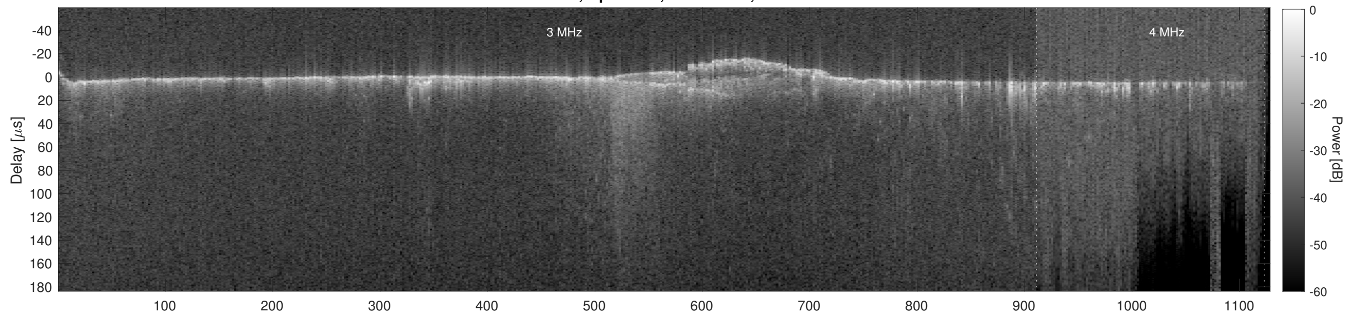
Orbit 14010, Cluttergram
