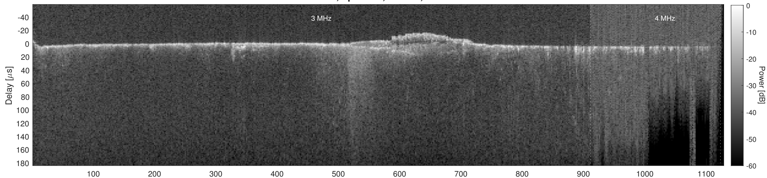
Orbit 14010, Cluttergram
