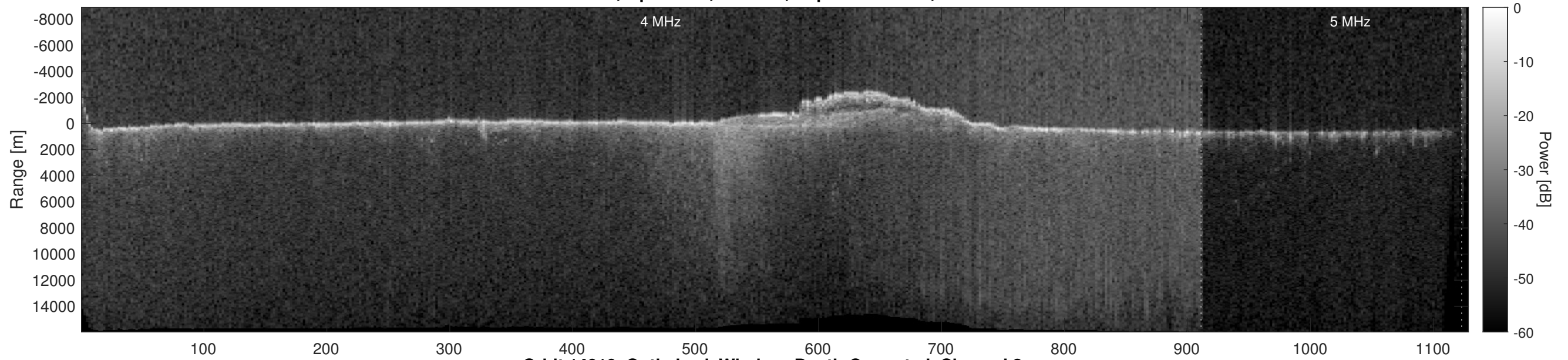
Orbit 14010, Optimized, Window, Depth-Corrected, Channel 2
