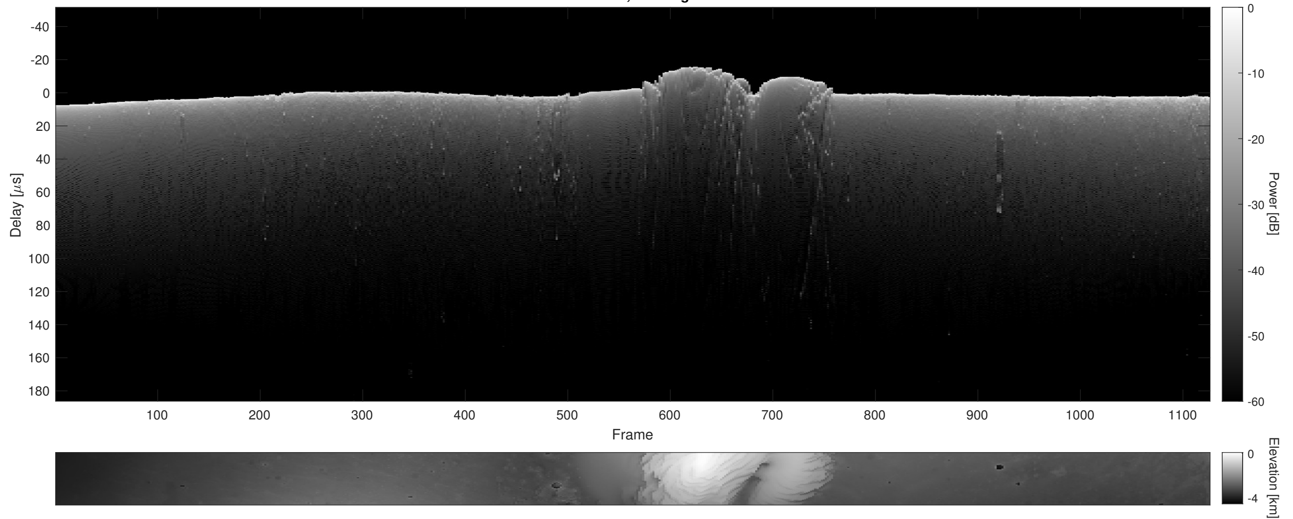
Orbit 14013, Cluttergram
