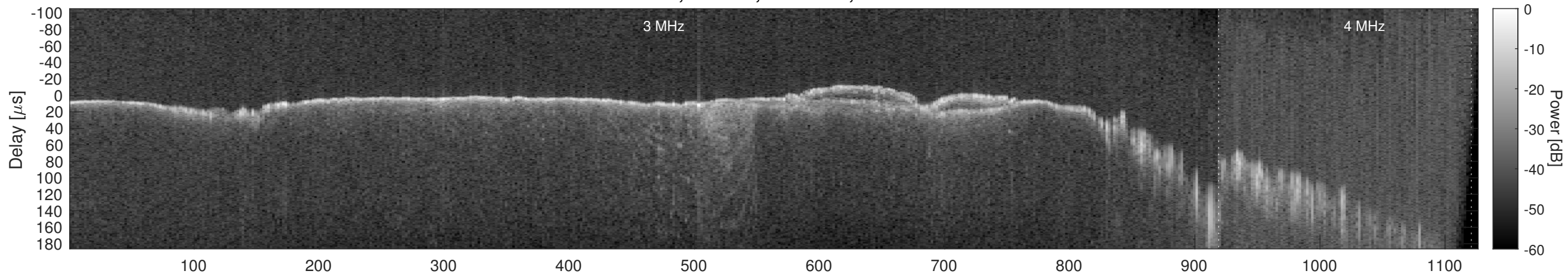
Orbit 14013, Window, Channel 2, Chapman
