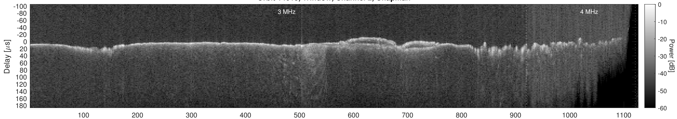
Orbit 14013, Window, Channel 2, Optimized
