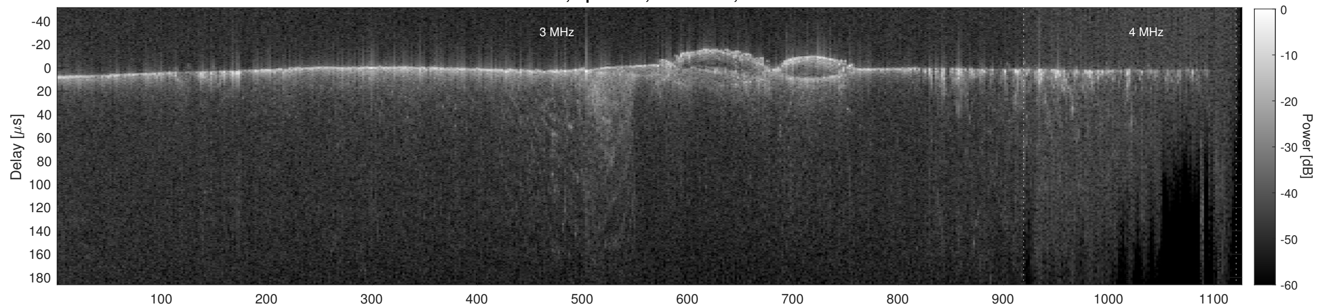
Orbit 14013, Cluttergram
