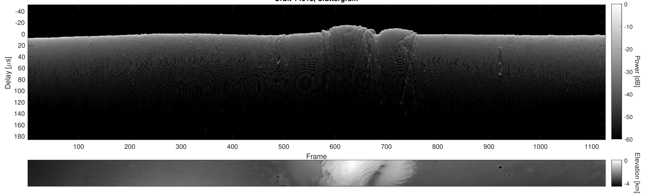
Orbit 14013, Cluttergram
