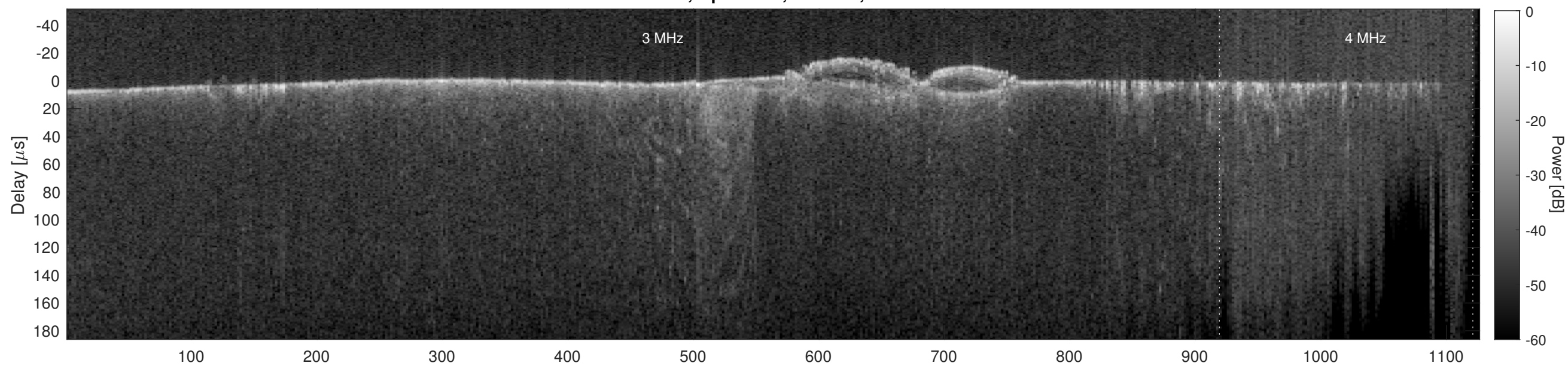
Orbit 14013, Cluttergram
