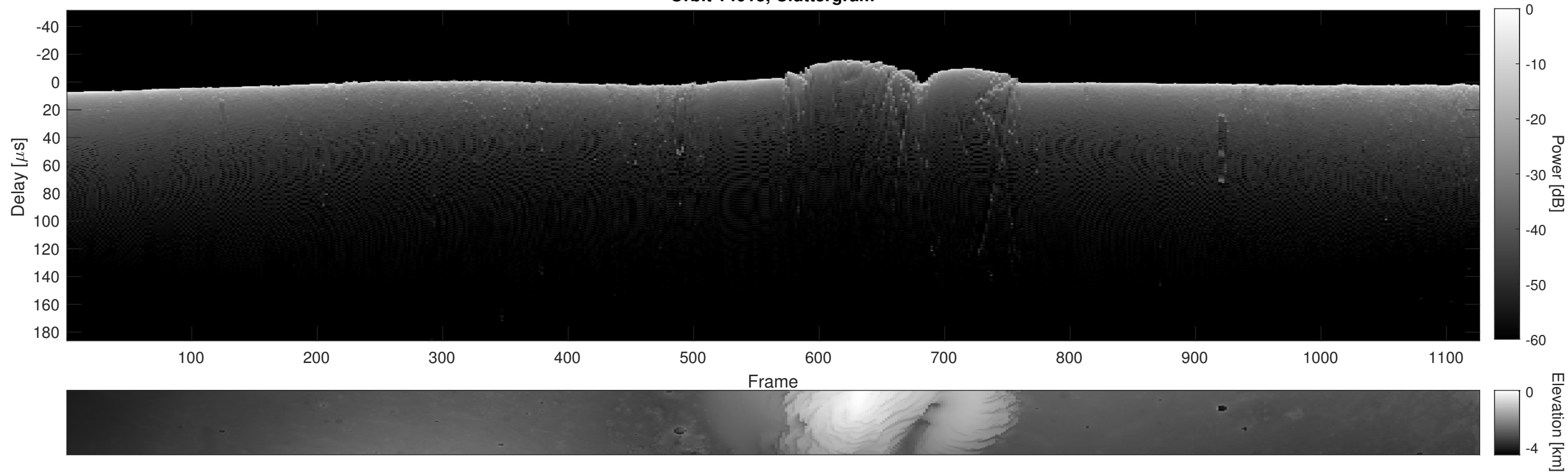
Orbit 14013, Cluttergram
