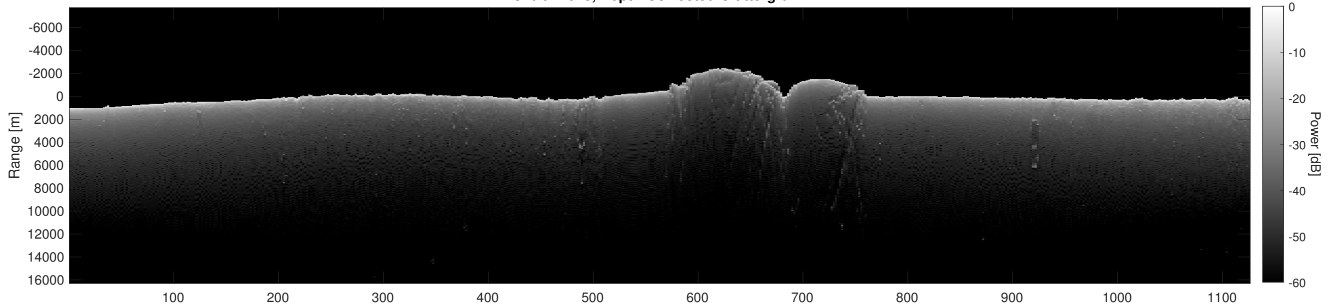
Orbit 14013, Depth-Corrected Cluttergram
