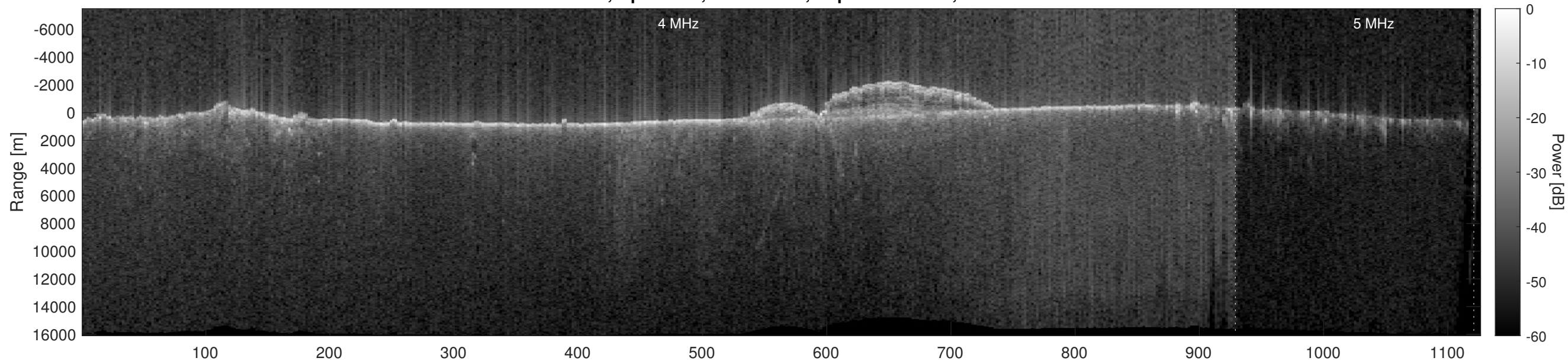
Orbit 14019, Optimized, No Window, Depth-Corrected, Channel 2
