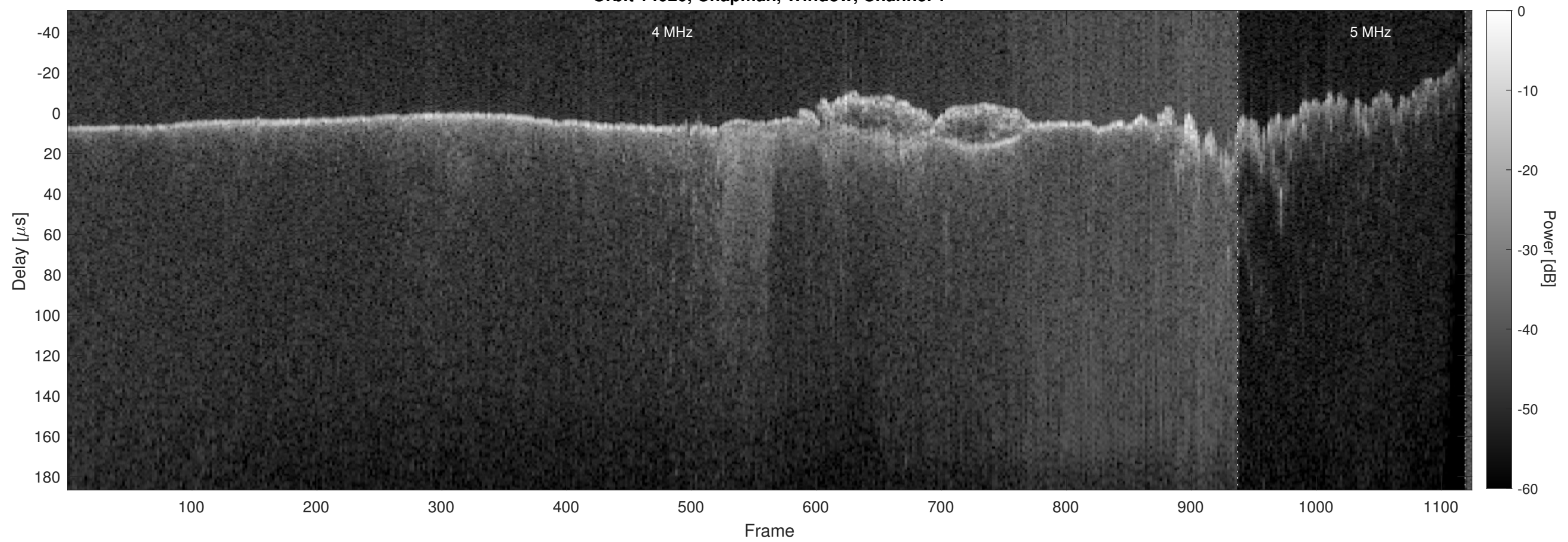
Orbit 14020, Chapman, Window, Channel 2
