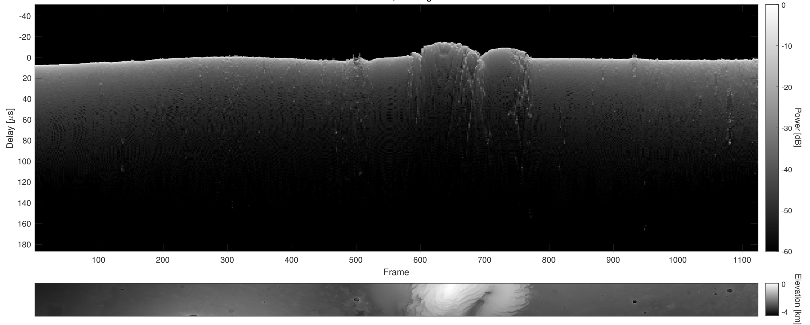
Orbit 14020, Cluttergram
