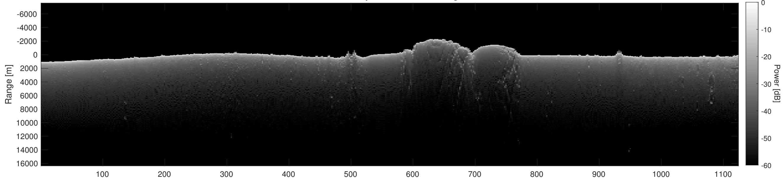
Orbit 14020, Depth-Corrected Cluttergram
