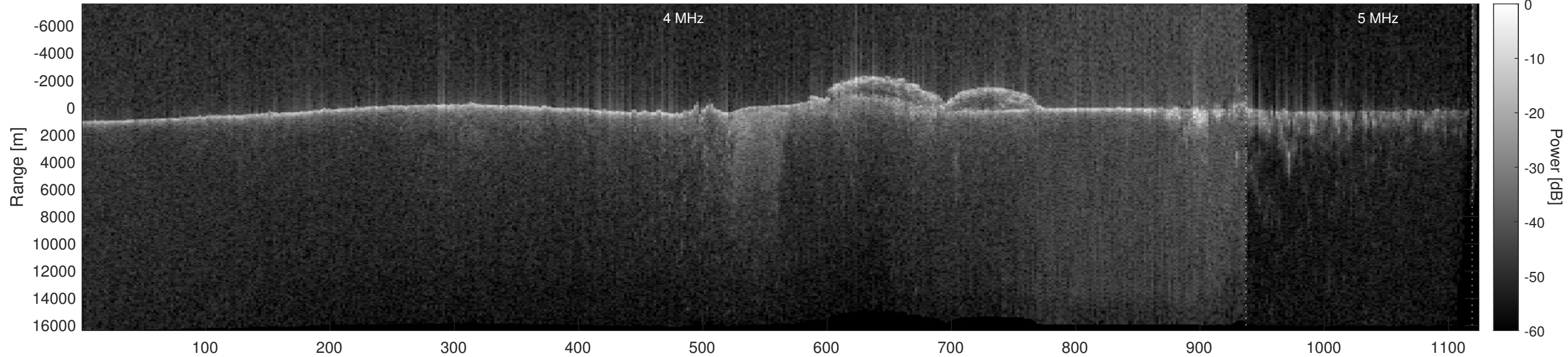
Orbit 14020, Optimized, No Window, Depth-Corrected, Channel 2
