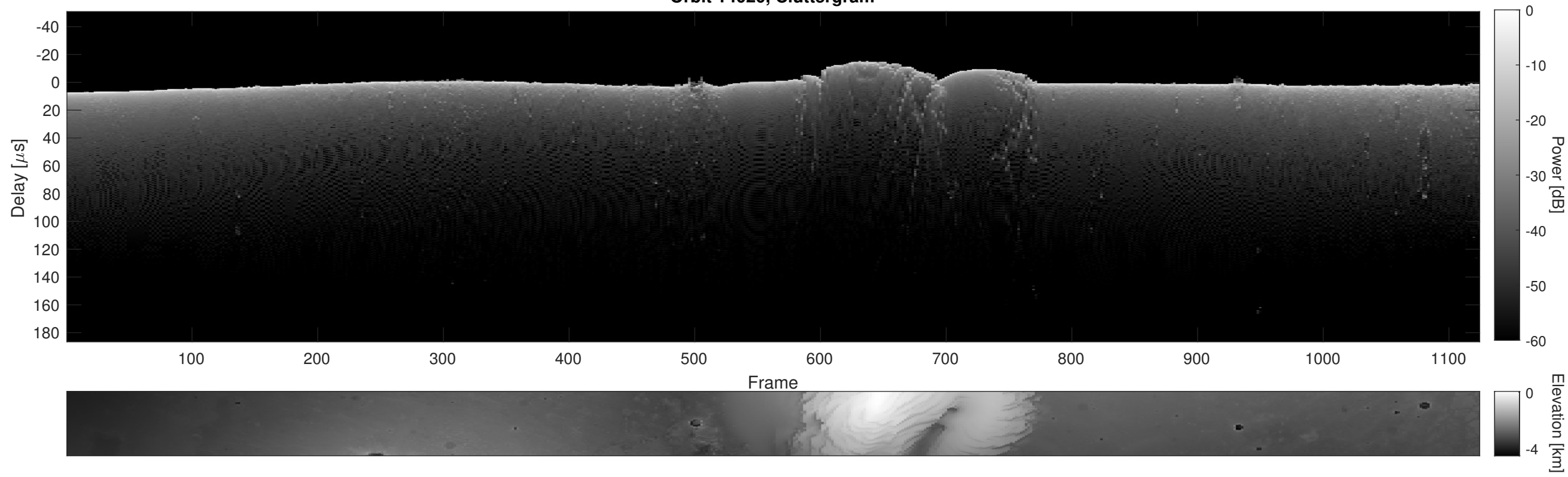
Orbit 14020, Cluttergram
