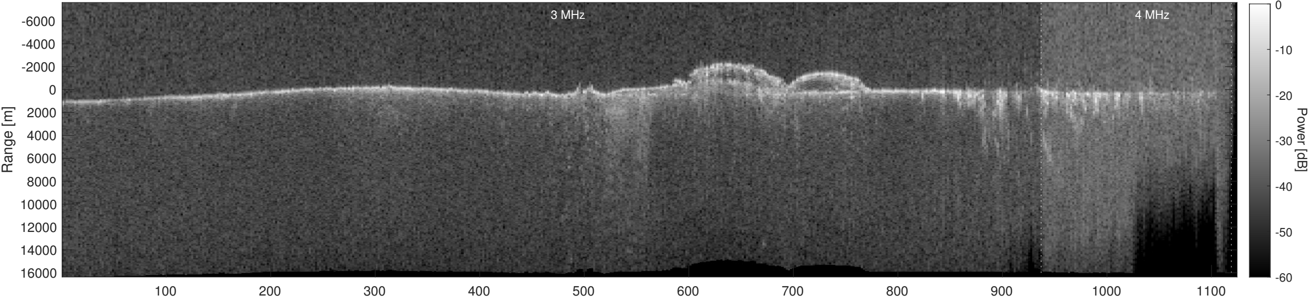
Orbit 14020, Depth-Corrected Cluttergram
