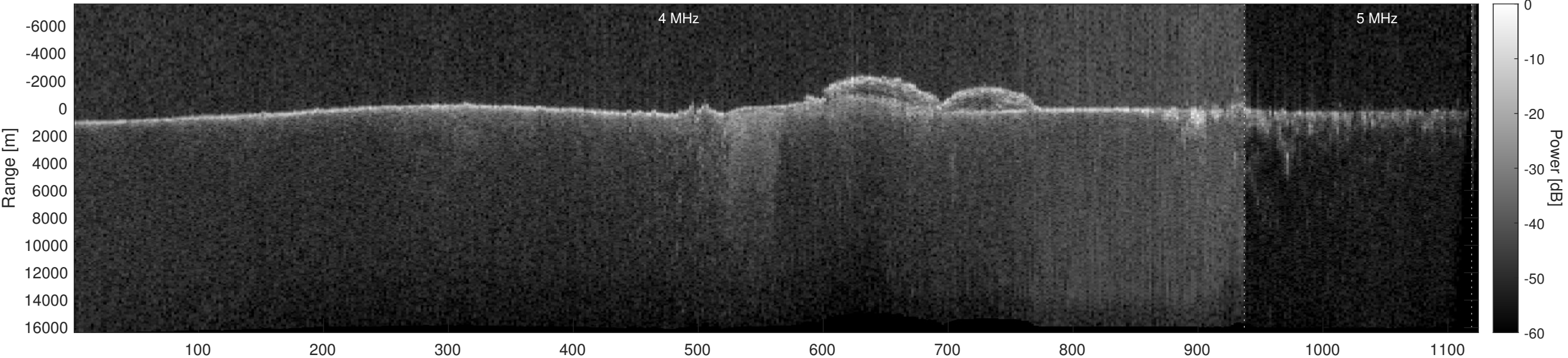
Orbit 14020, Optimized, Window, Depth-Corrected, Channel 2
