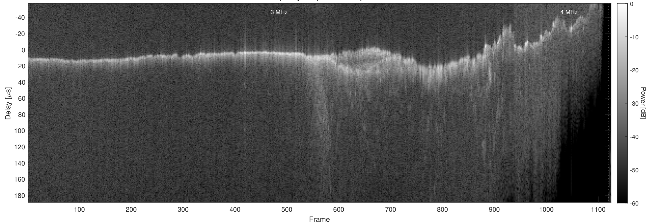
Orbit 14021, Chapman, No Window, Channel 2
