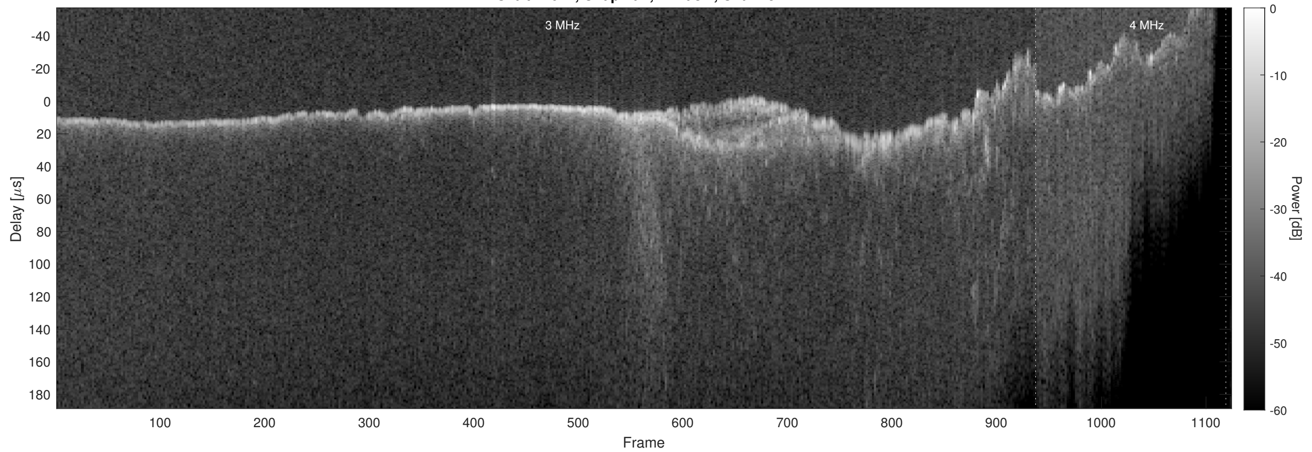
Orbit 14021, Chapman, Window, Channel 2
