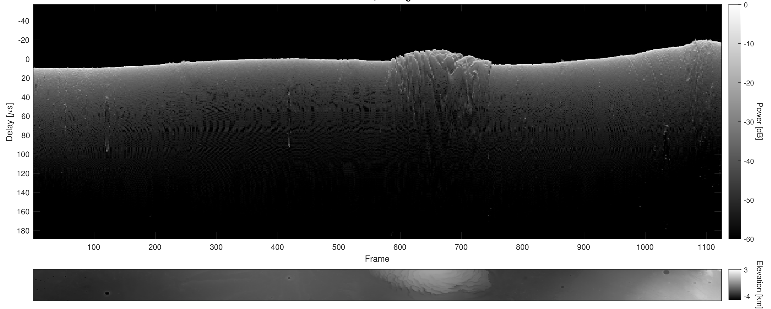
Orbit 14021, Cluttergram
