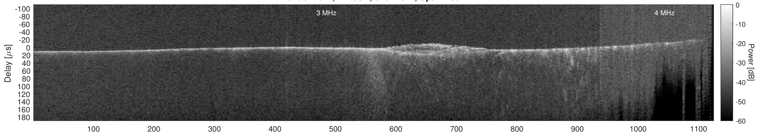
Orbit 14021, Cluttergram
