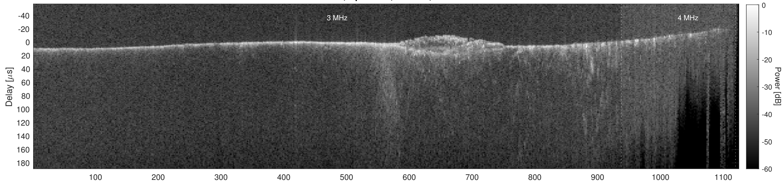
Orbit 14021, Cluttergram
