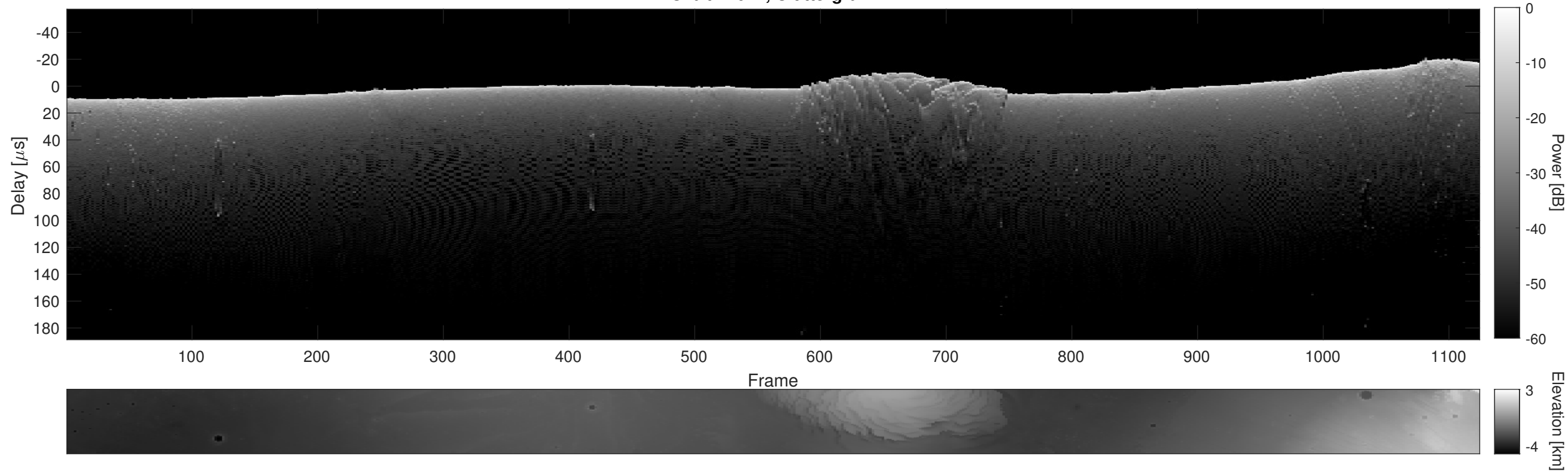
Orbit 14021, Cluttergram
