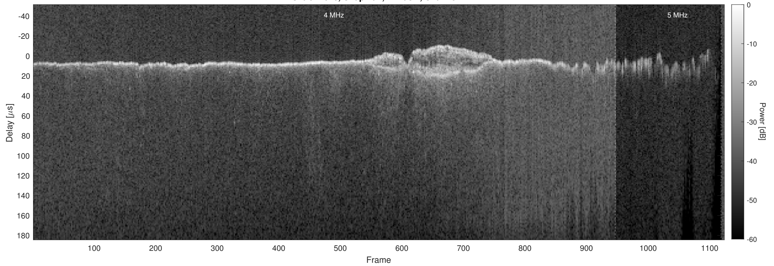
Orbit 14026, Chapman, Window, Channel 2
