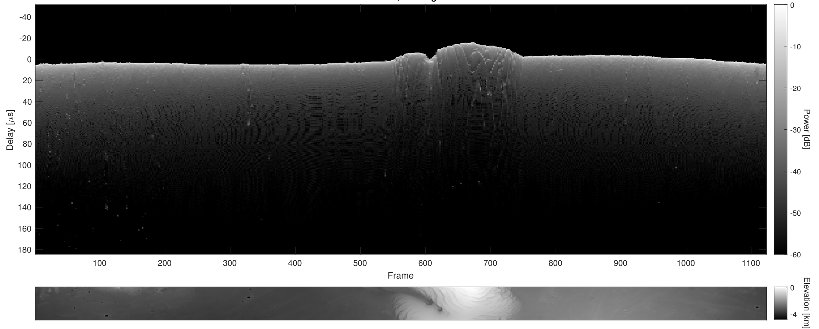
Orbit 14026, Cluttergram
