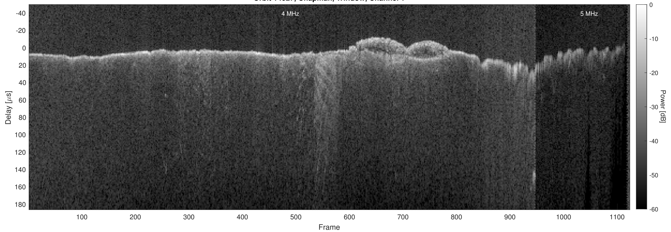
Orbit 14027, Chapman, Window, Channel 2
