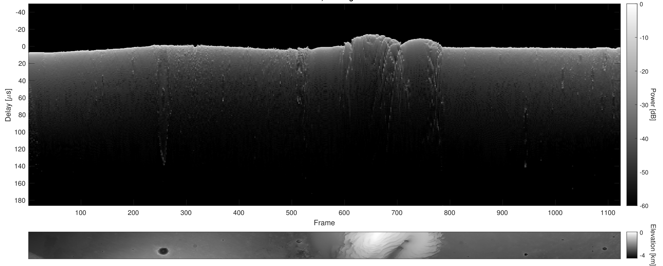
Orbit 14027, Cluttergram
