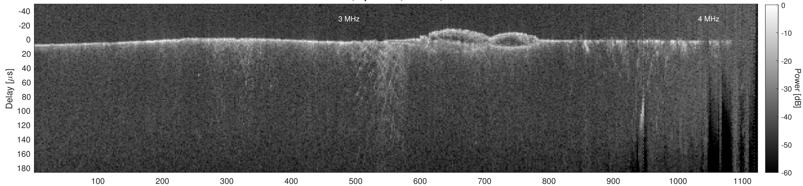
Orbit 14027, Cluttergram
