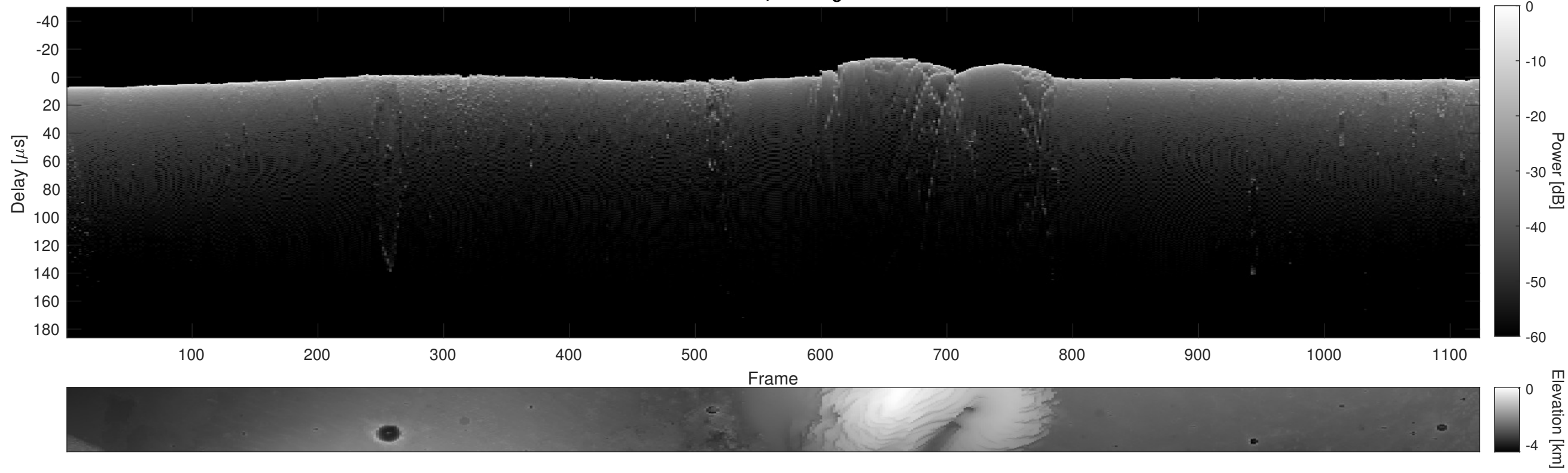
Orbit 14027, Cluttergram
