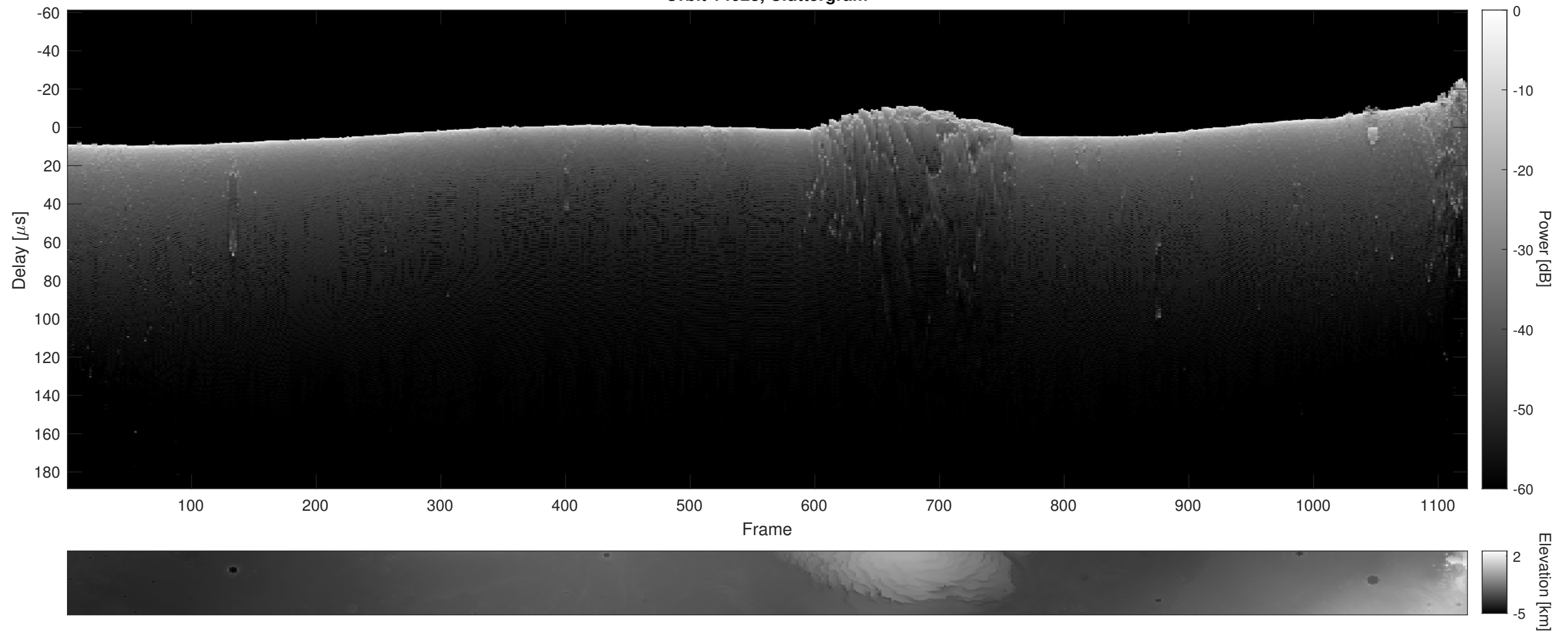
Orbit 14028, Cluttergram
