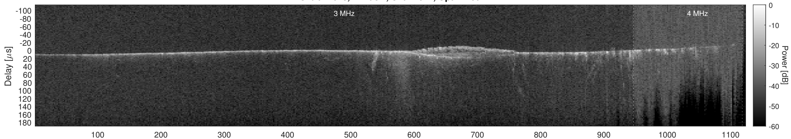
Orbit 14028, Cluttergram
