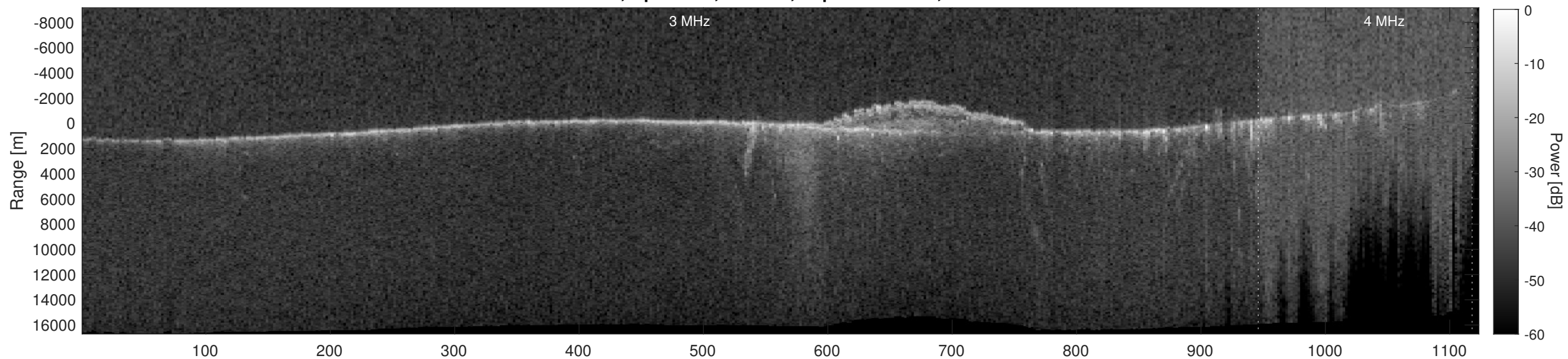
Orbit 14028, Depth-Corrected Cluttergram
