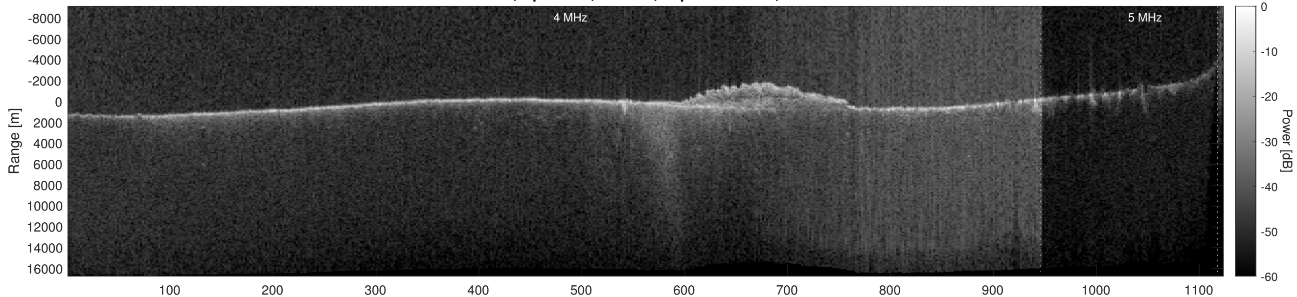
Orbit 14028, Optimized, Window, Depth-Corrected, Channel 2
