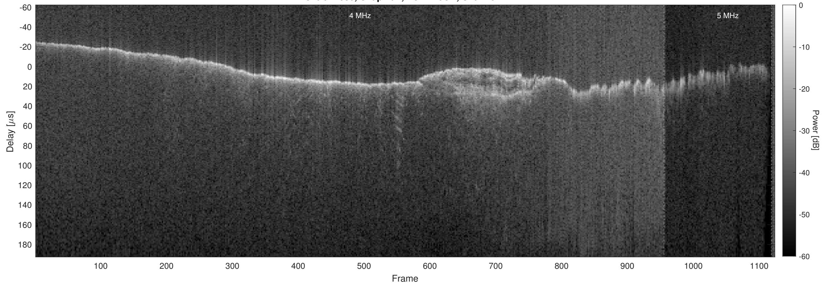
Orbit 14030, Chapman, No Window, Channel 2
