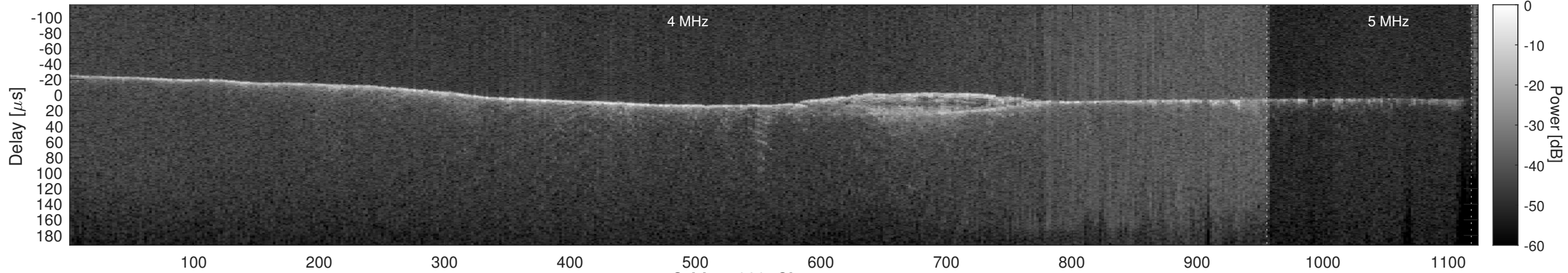
Orbit 14030, Cluttergram
