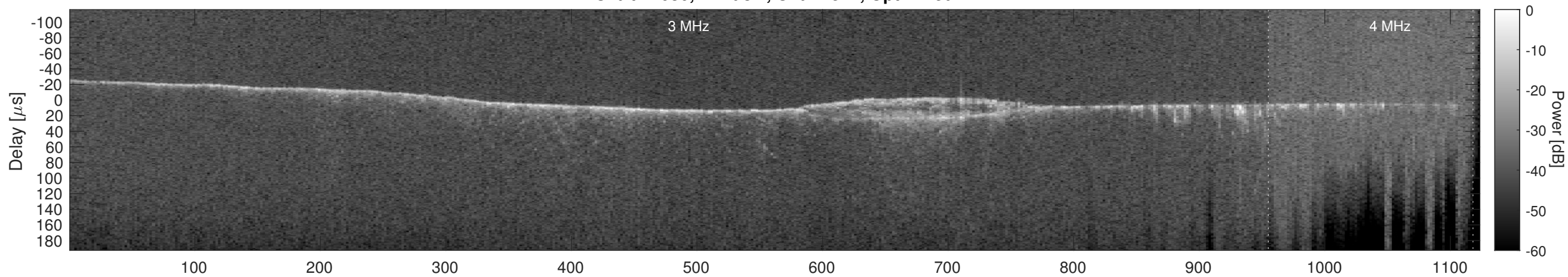
Orbit 14030, Cluttergram
