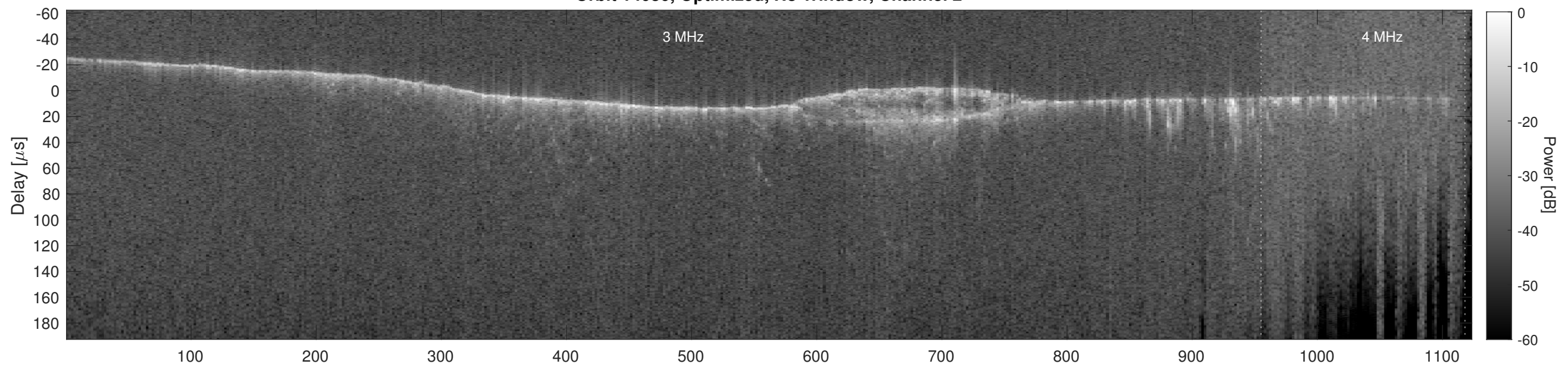
Orbit 14030, Cluttergram
