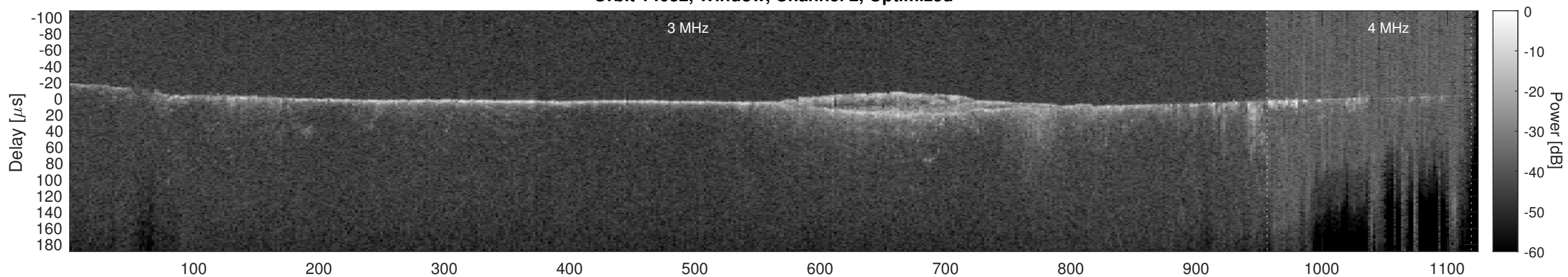
Orbit 14032, Cluttergram
