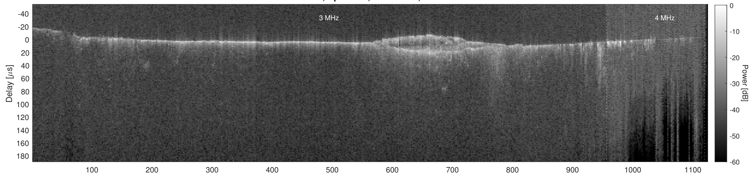
Orbit 14032, Cluttergram
