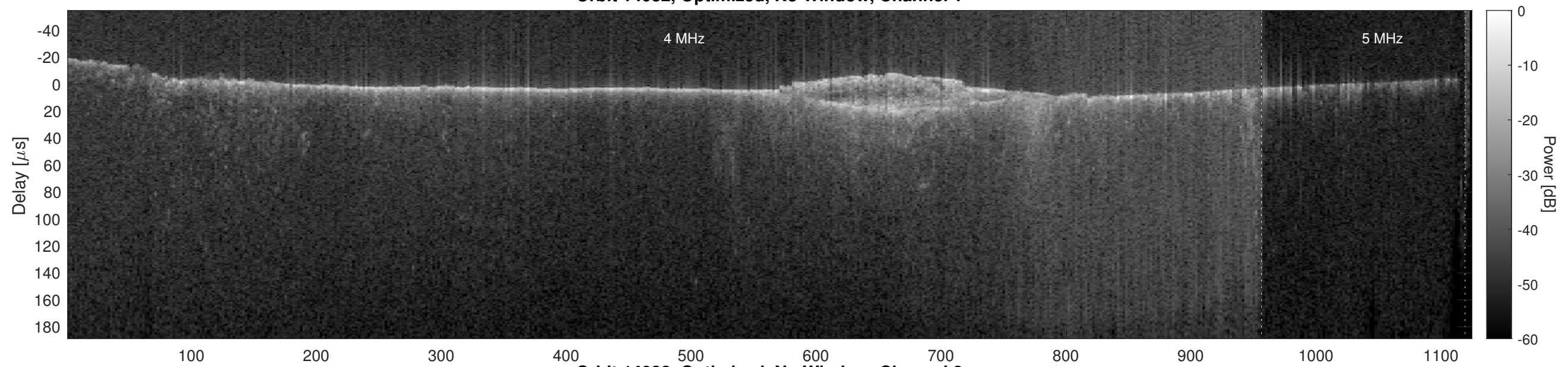
Orbit 14032, Optimized, No Window, Channel 2
