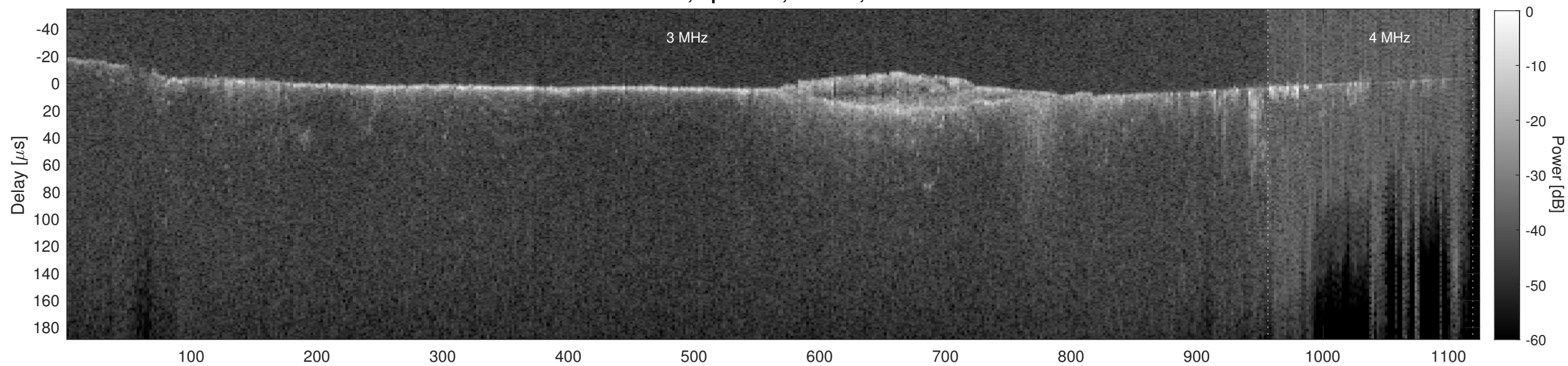
Orbit 14032, Cluttergram
