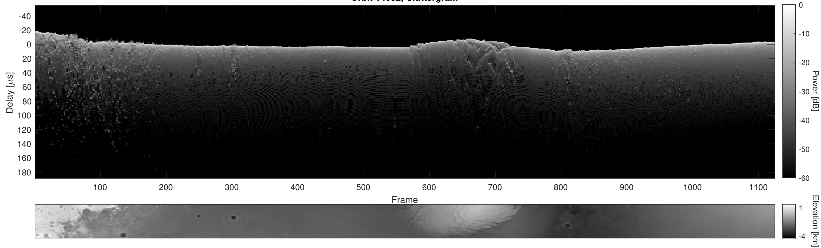
Orbit 14032, Cluttergram
