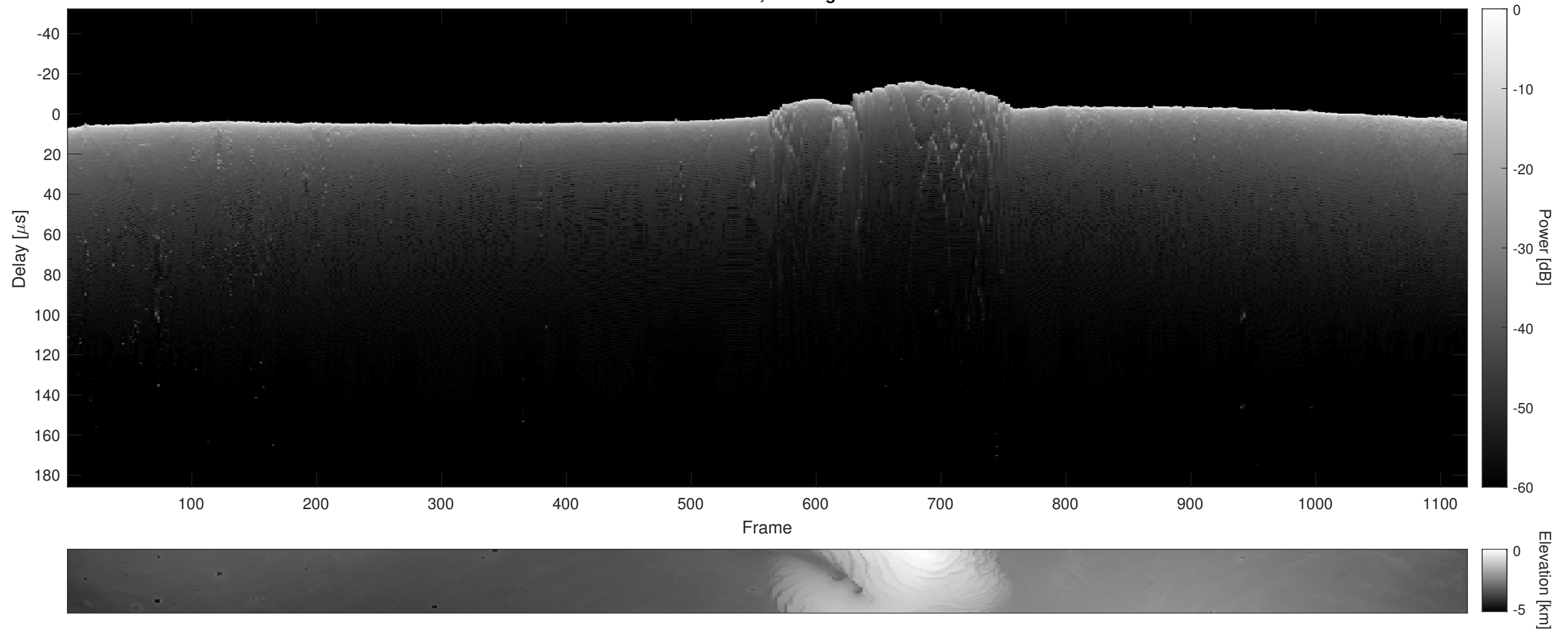
Orbit 14033, Cluttergram
