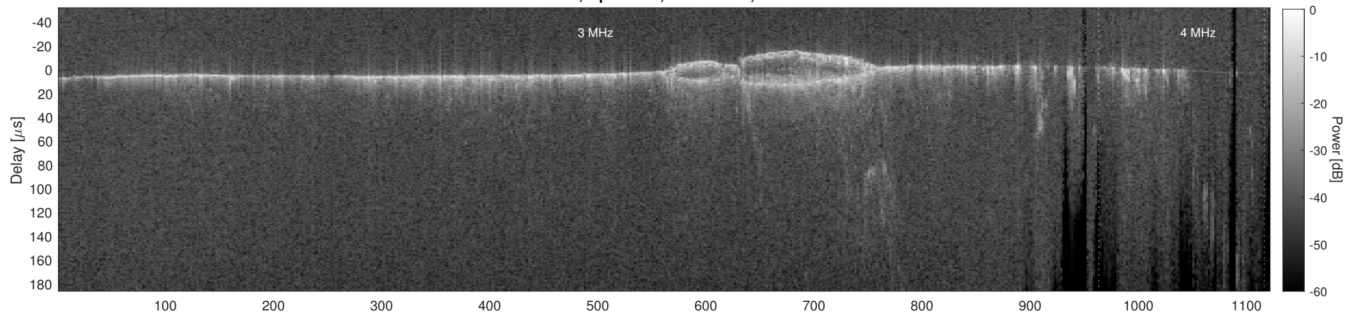
Orbit 14033, Cluttergram
