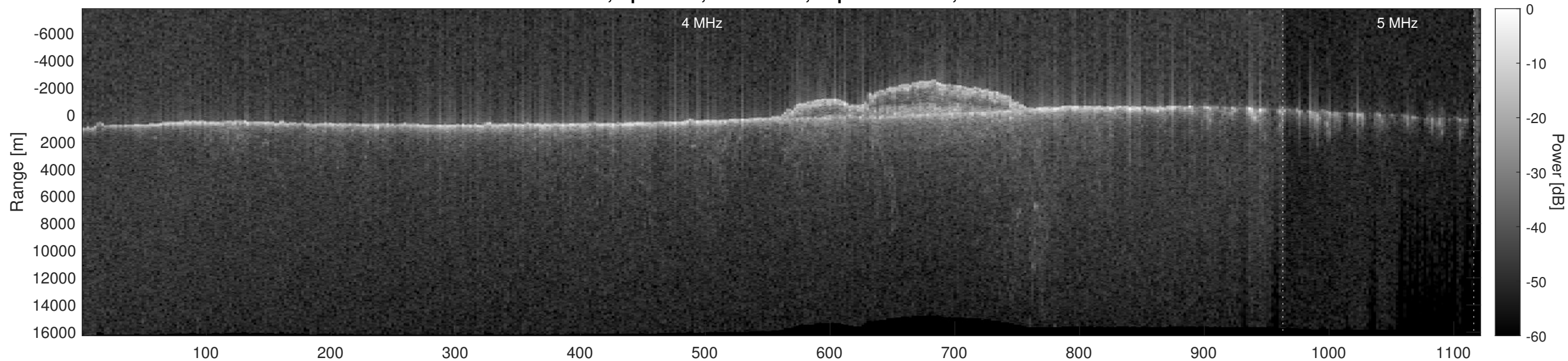
Orbit 14033, Optimized, No Window, Depth-Corrected, Channel 2
