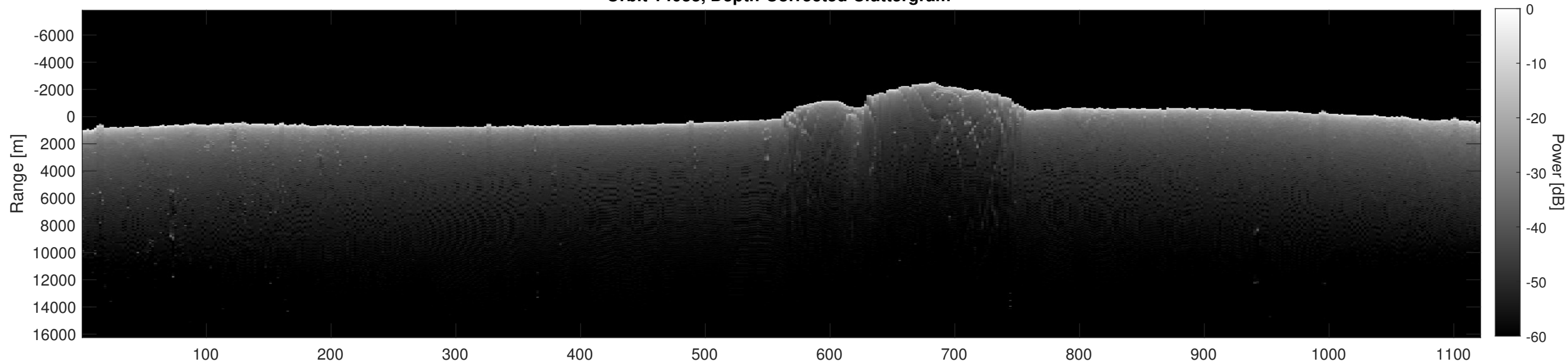
Orbit 14033, Depth-Corrected Cluttergram
