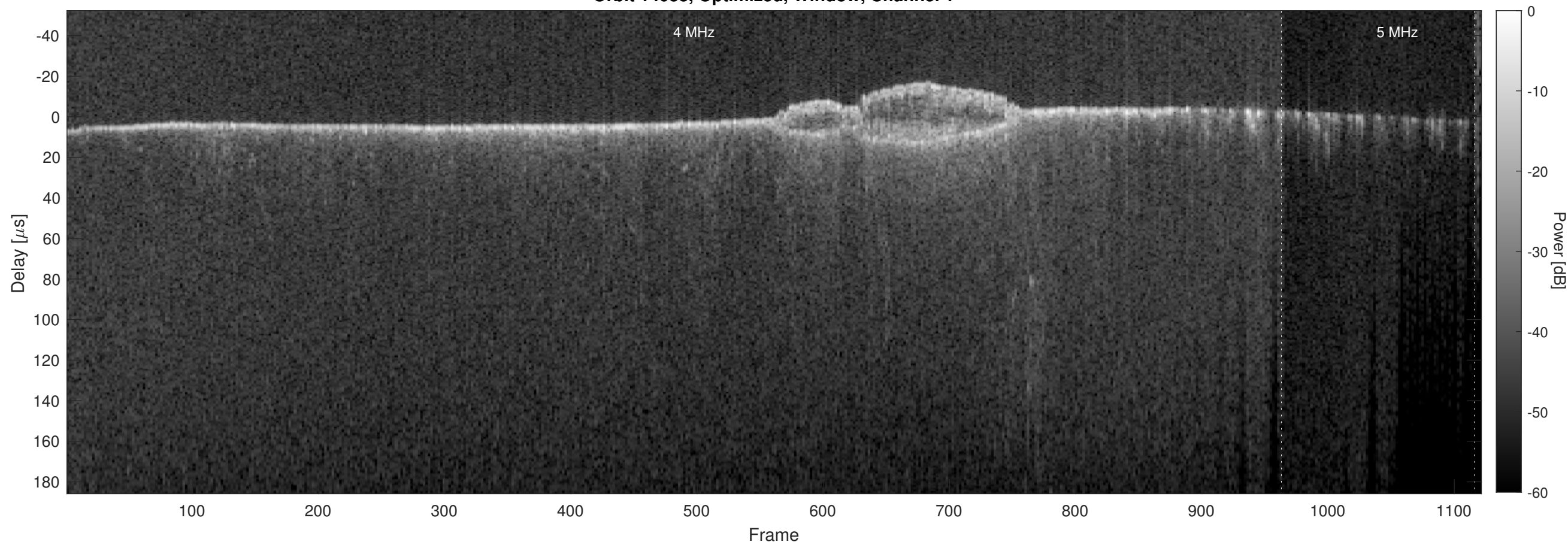
Orbit 14033, Optimized, Window, Channel 2
