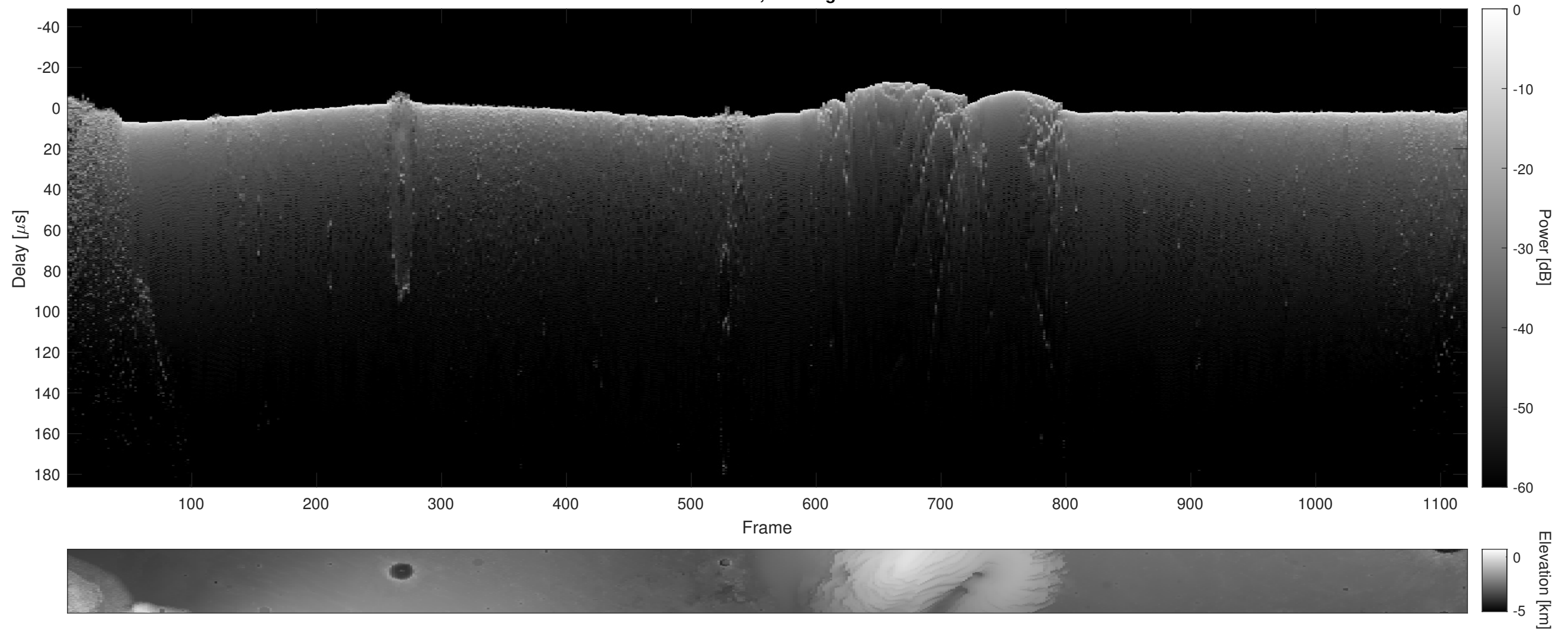
Orbit 14034, Cluttergram
