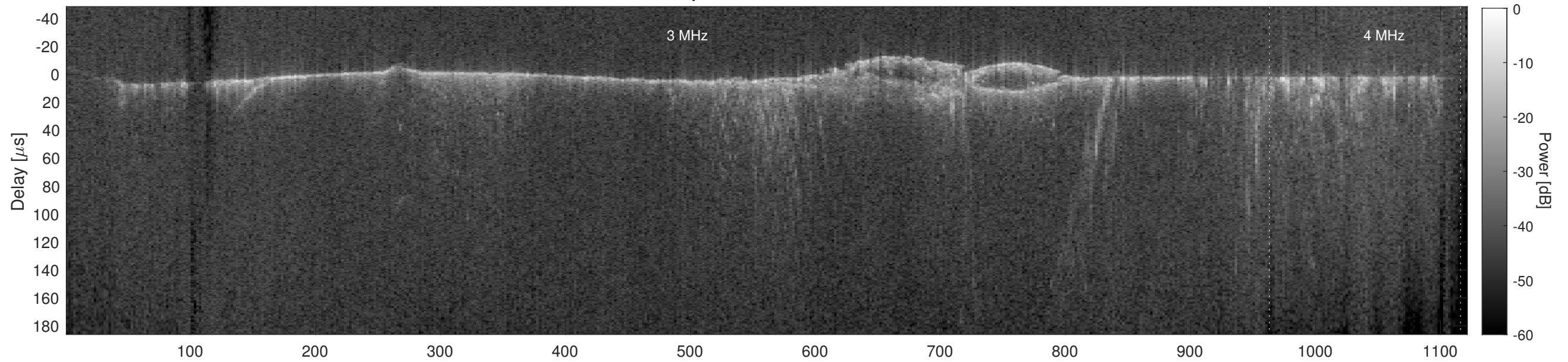
Orbit 14034, Cluttergram
