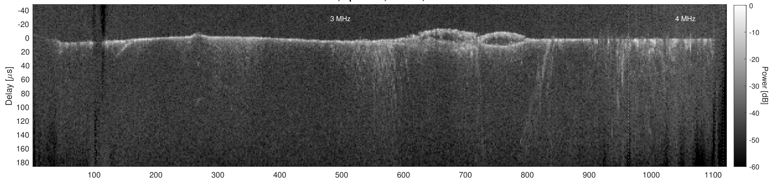
Orbit 14034, Cluttergram
