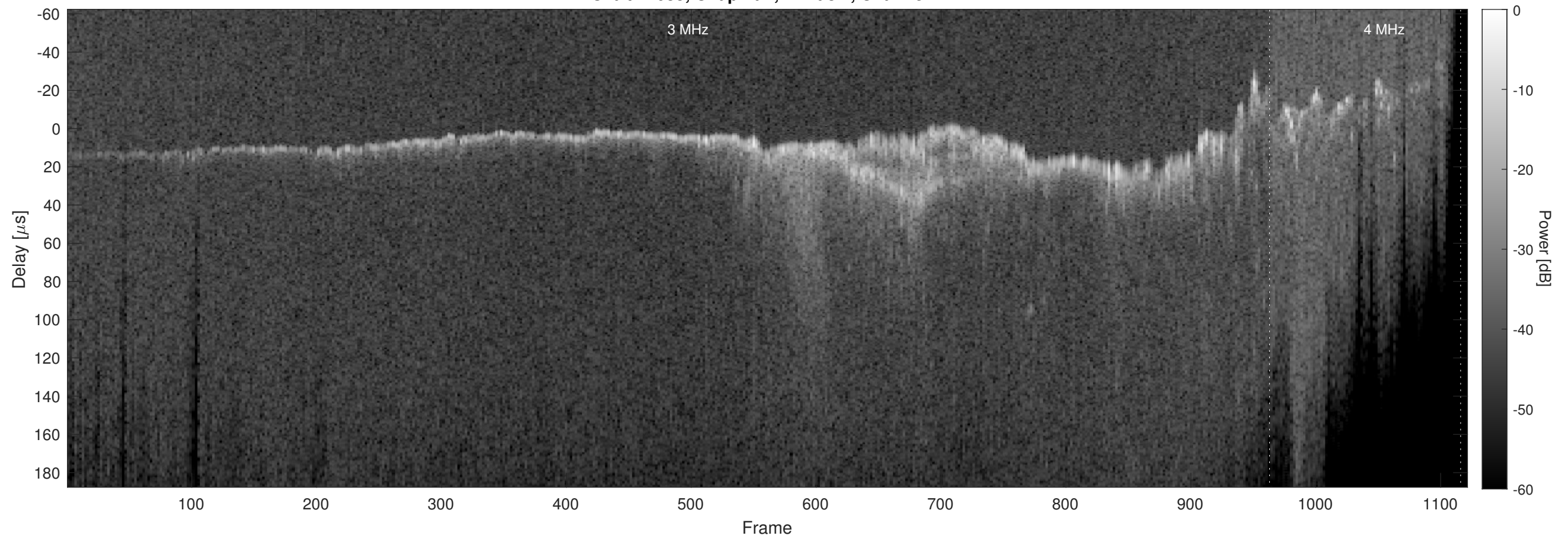
Orbit 14035, Chapman, Window, Channel 2
