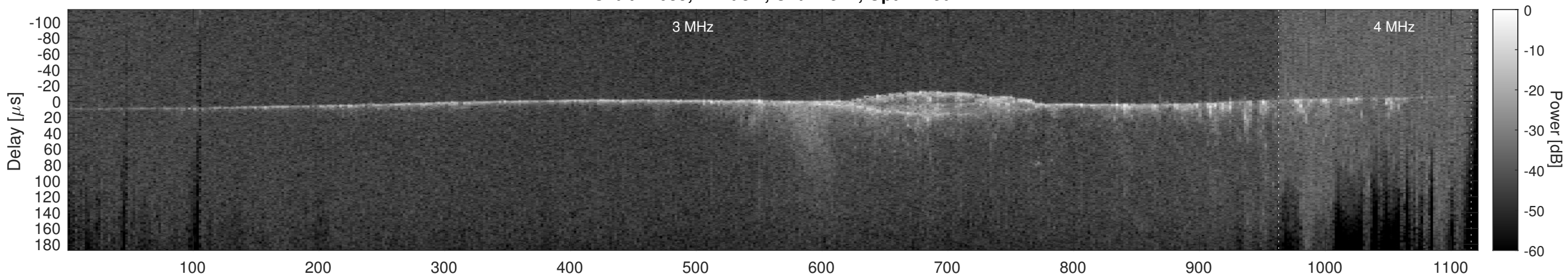
Orbit 14035, Cluttergram
