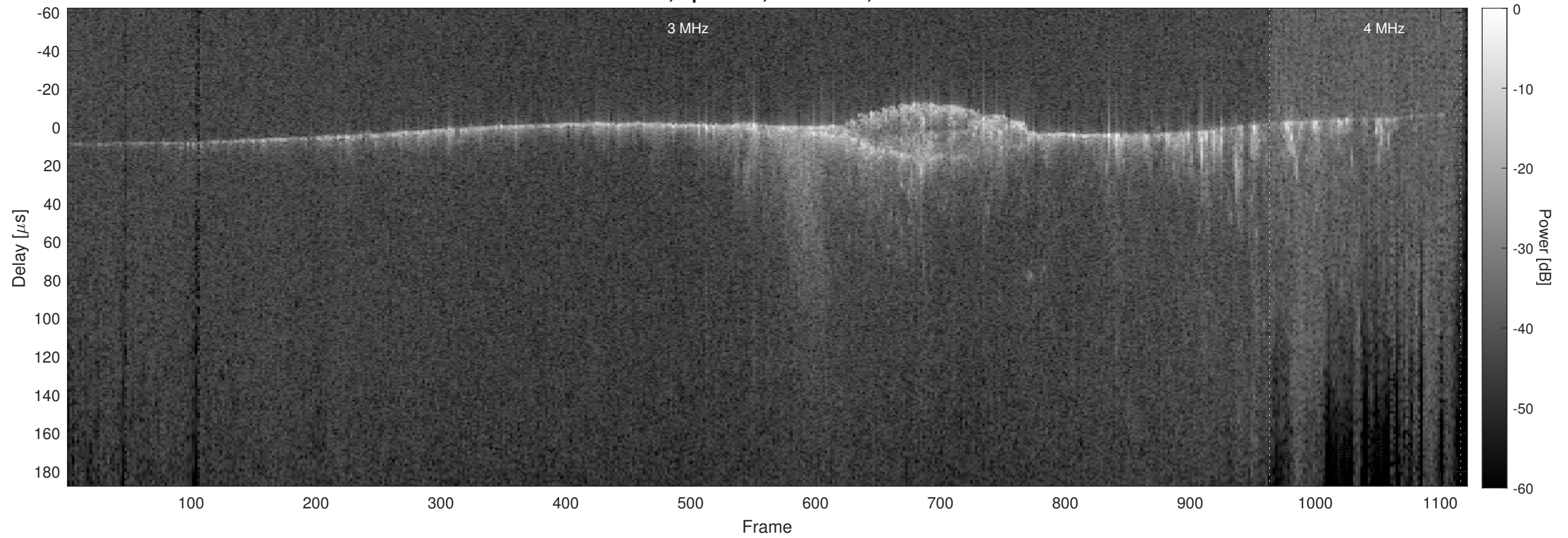
Orbit 14035, Optimized, No Window, Channel 2
